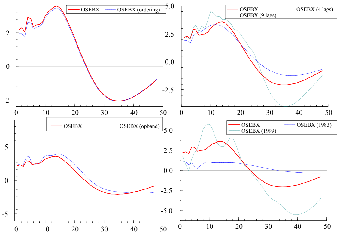
Figure 4 Robustness of responses in stock return (OSEBX) to an oil price shock, percentage a)
